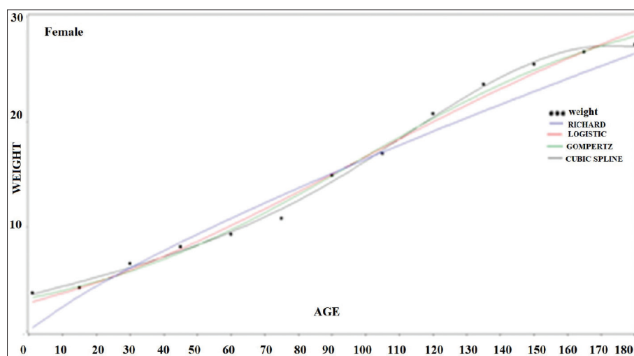
Fig 1. Growth curves of the female lambs by different growth functions
