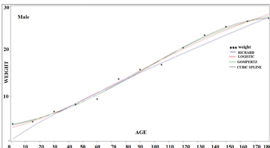
Fig 2. Growth curves of the male lambs by different growth functions
