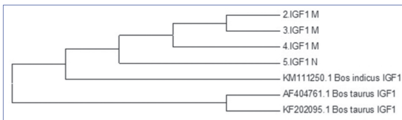
Fig 13. Phylogenetic tree of the IGF1 gene sequences of Baggara, Bos taurus and Bos indicus cattle. M: Mesairi strain, N: Nyalawi strain
