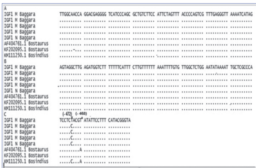
Fig 12. Comparison of the IGF1 gene sequences of Baggara, Bos taurus (AF404761 and KF202095) and Bos indicus cattle (KM111250). M: Mesairi strain. N: Nyalawi strain. Aligned sequences of partial 5' UTR are presented in 3 patches and given the letters A, B, & C
