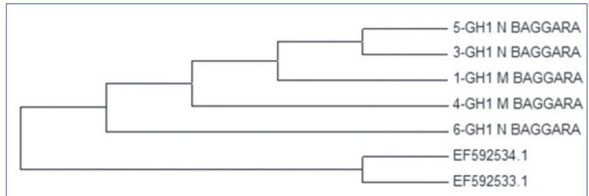
Fig 8. Phylogenetic tree of the GH1 gene sequences of Baggara, Kenana (EF592534.1) and Butana (EF592533.1) cattle
