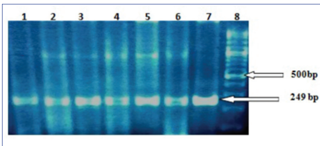
Fig 9. Agarose gel electrophoresis (2%) displaying PCR amplification of Baggara IGF1 5'-flanking region. Lanes: 1-7 PCR products of samples. Lane 8: 100 bp DNA Ladder
