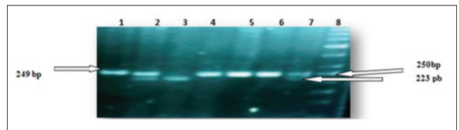
Fig 10. Agarose gel electrophoresis (2%) displaying SnaBI restriction digest of an amplified portion of Baggara IGF1 gene in the 5'-flanking region. Lanes: 1, 4, 5 and 6 representing CC genotype (249 bp). Lane 3 representing TT genotype (223+26). Lanes 2 and 7 representing CT genotype (249+223+26). Lane 8: 50 bp DNA ladder
